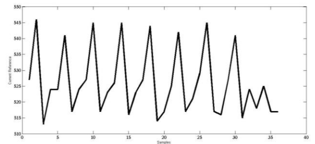
FIGURE 20. Current Consumption (mA) of the ELS Mechanism
