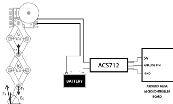
FIGURE 18. Current Measurement Setup of the two Mechanisms (only ELS Mechanism shown)
